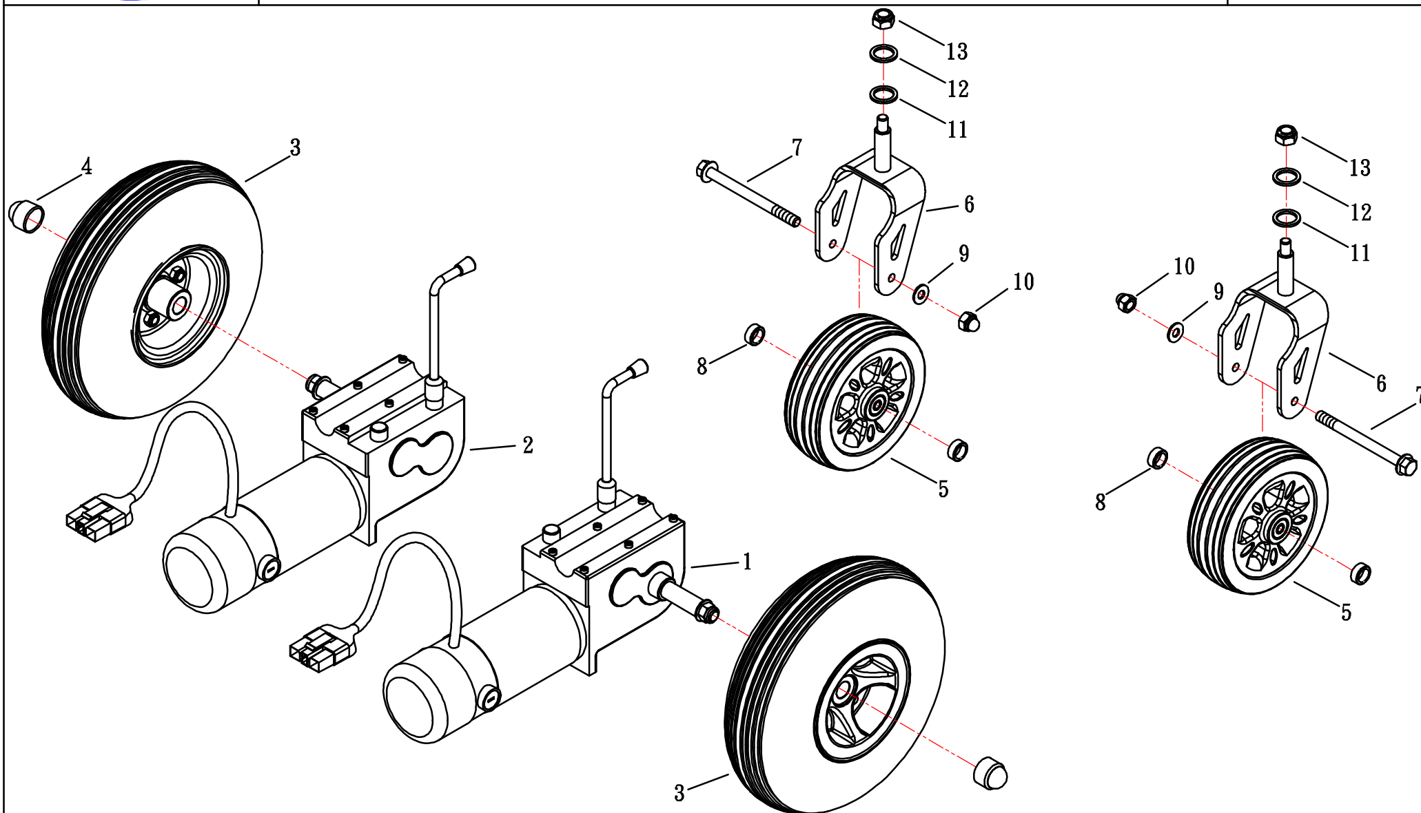
(FIG. 5) WHEEL
